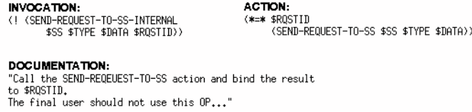
Figure 4.9: A Standard Action OP
