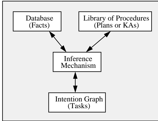
Figure 1: OPRS Global Architecture
